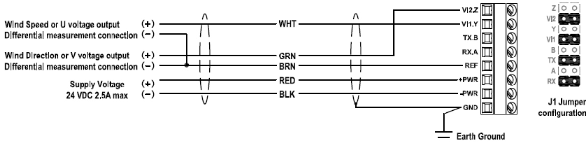
Fig. A2: 4-20 mA CURRENT OUTPUT
